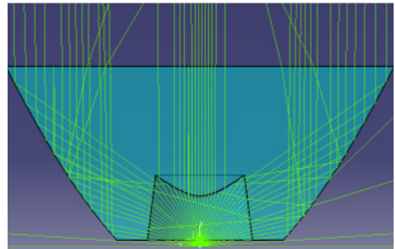
TIR Optics Allow for Precise Beam Control Without Halo Effect
