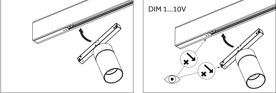
MOUNTING PROJECTOR
