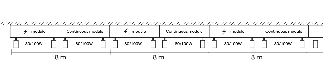
ELECTRICAL CAPACITY TRACELINE TRACK 48V SURFACE-PENDANT*
