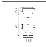
Ceiling clamp 0.02065.00
