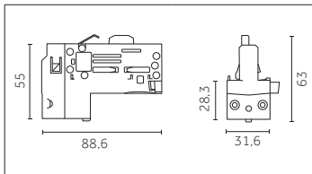
Technical data / Specifications: - frequency: 50Hz - nominal current and voltage: 6/10A-250V - polycarbonate body - copper alloy contacts - max. capacity: 100 N 0.02066.0000
