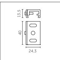
Ceiling bracket 0.02054.00
