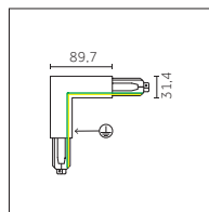
L-connector
